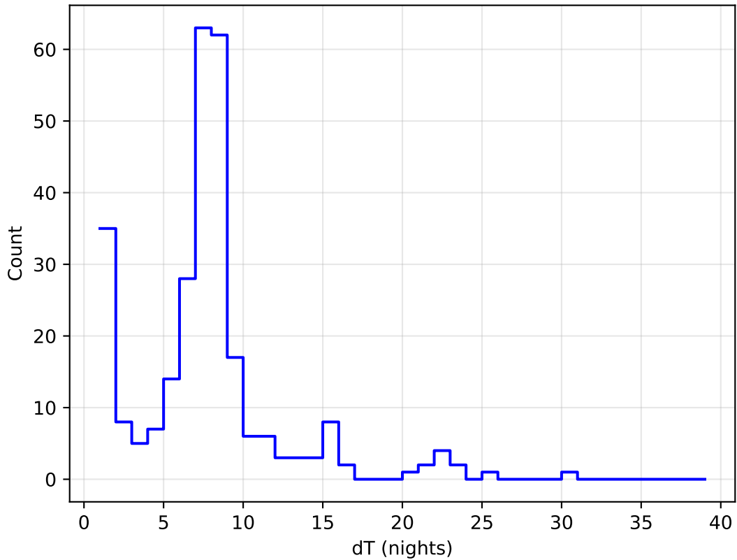
too_elab_r16_d2_griz_v3.4_10yrs all bands: DD:ECDFS Delta Nights Histogram
