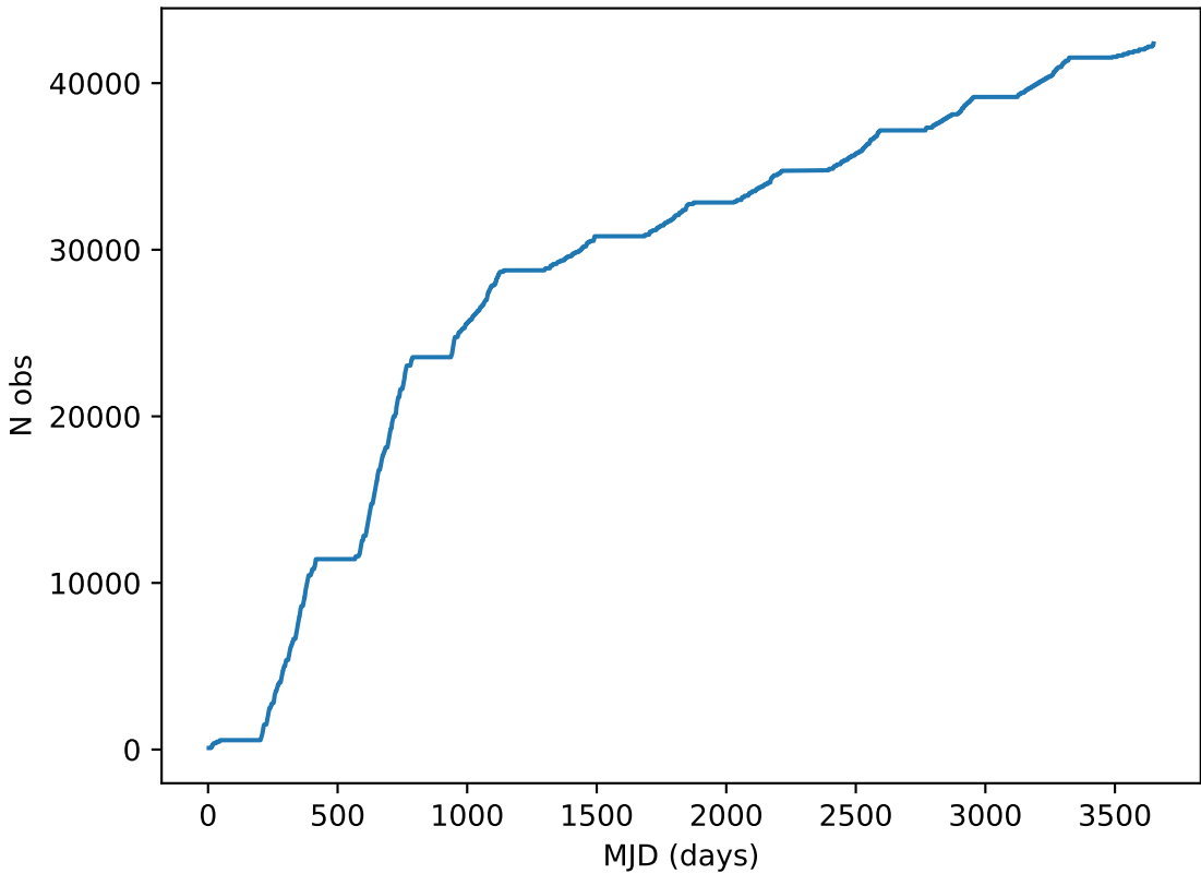
too_elab_r16_d2_griz_v3.4_10yrs all bands: DD: COSMOS Cumulative NVisits
