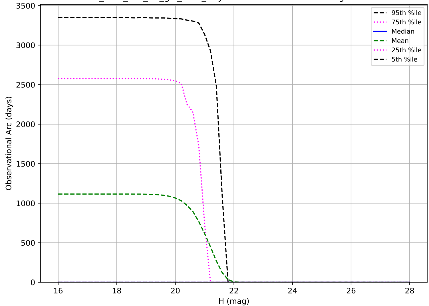
too_elab_r16_d2_giz_v3.4_10yrs: Observational Arc Length Vatira
