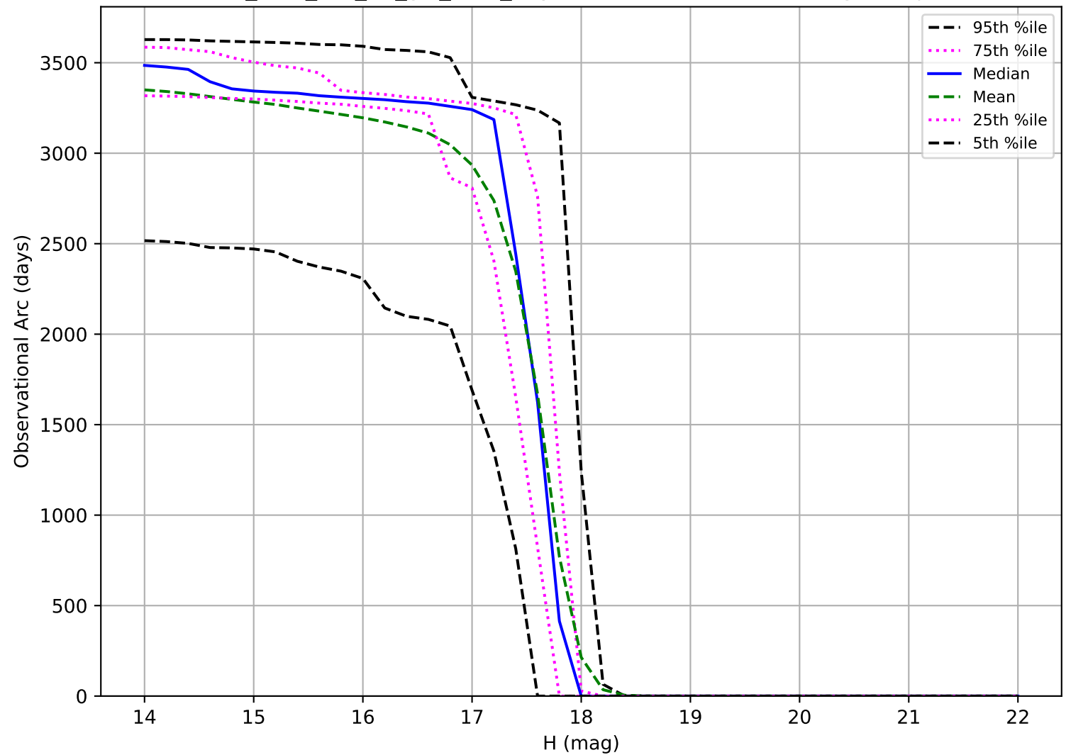
too_elab_r16_d2_giz_v3.4_10yrs: Observational Arc Length Trojan
