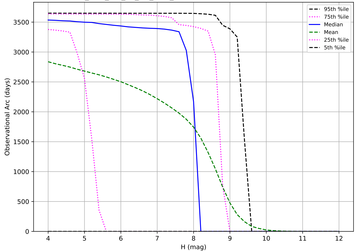
too_elab_r16_d2_giz_v3.4_10yrs: Observational Arc Length TNO
