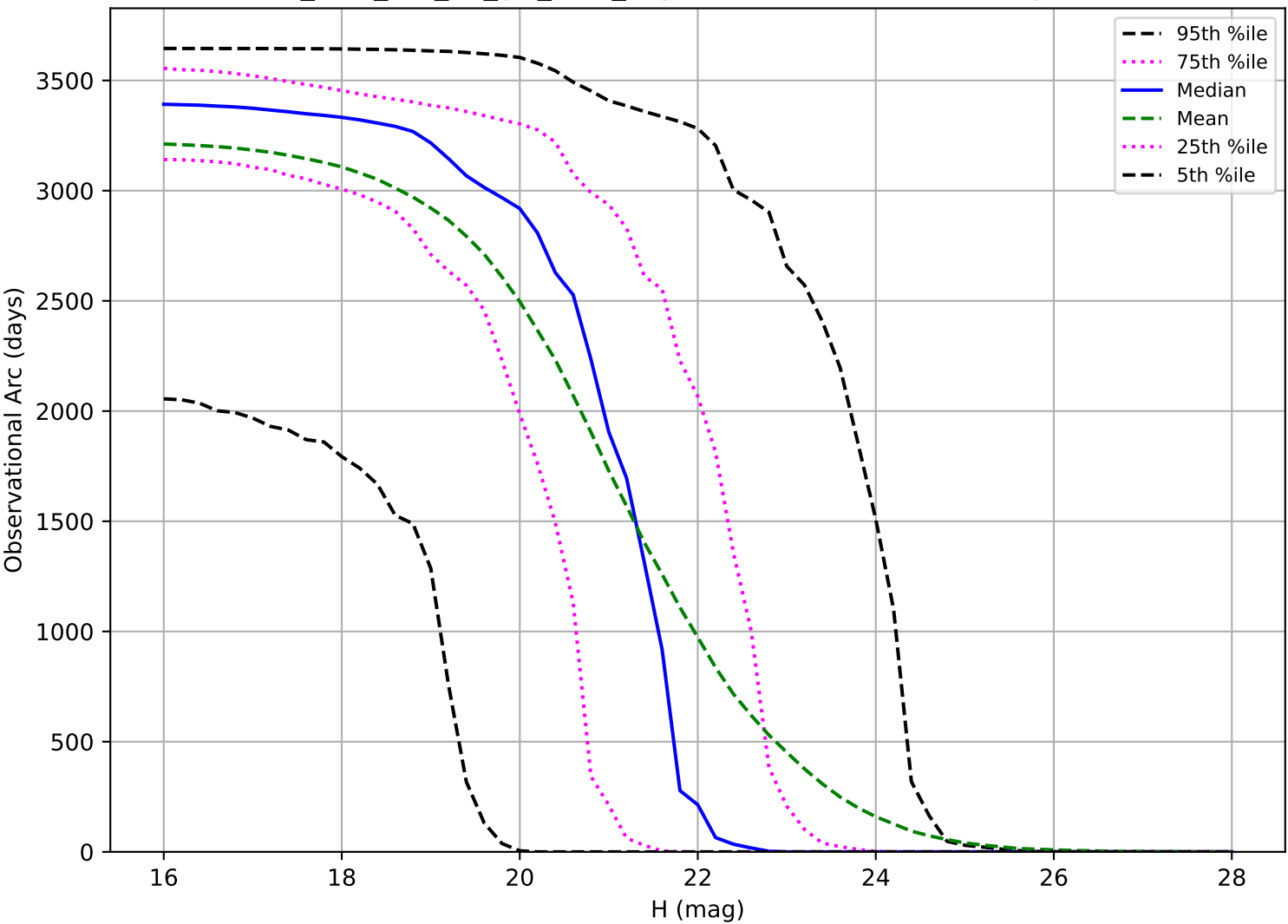
too_elab_r16_d2_giz_v3.4_10yrs: Observational Arc Length PHA
