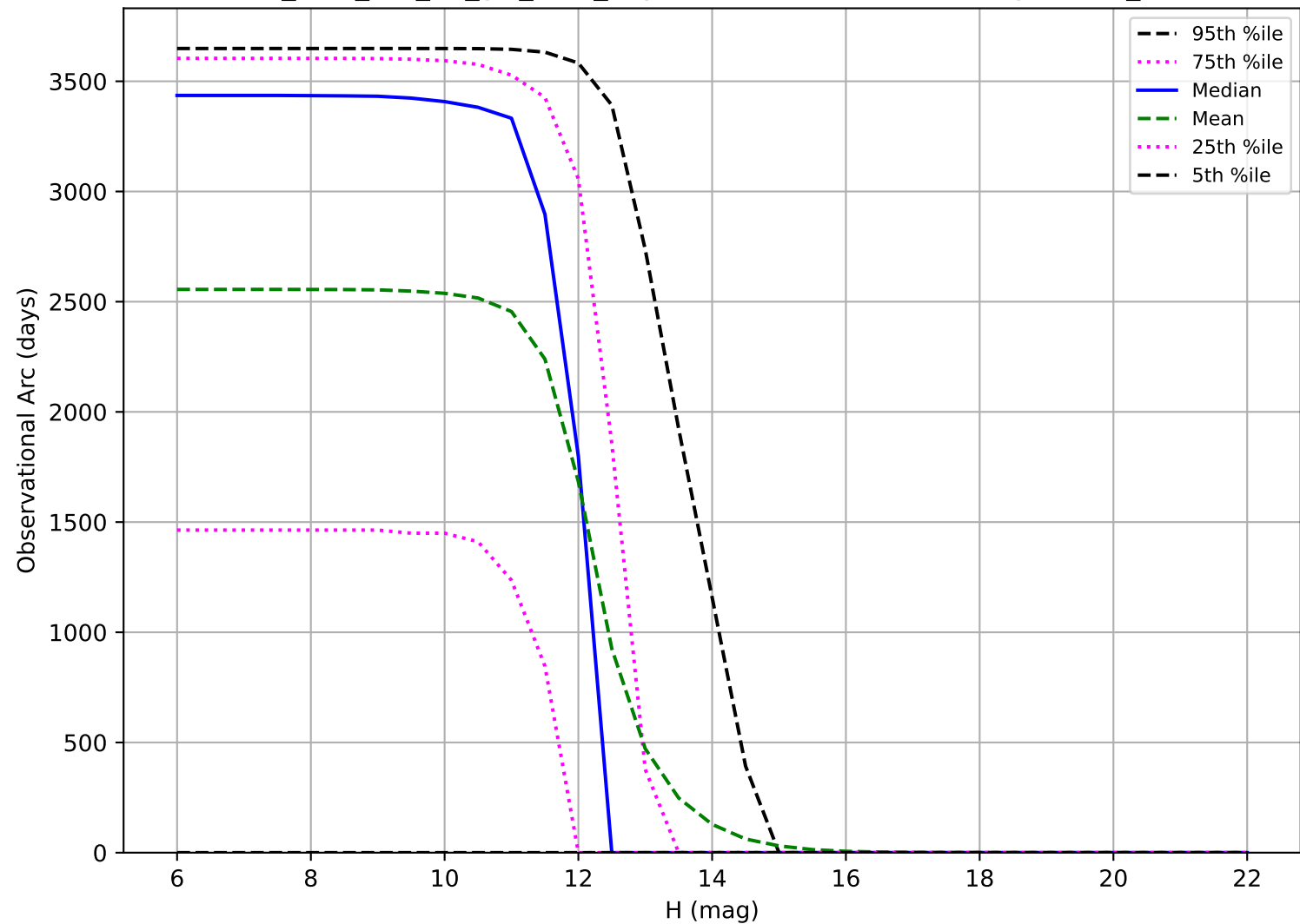
too_elab_r16_d2_giz_v3.4_10yrs: Observational Arc Length OCC_r20
