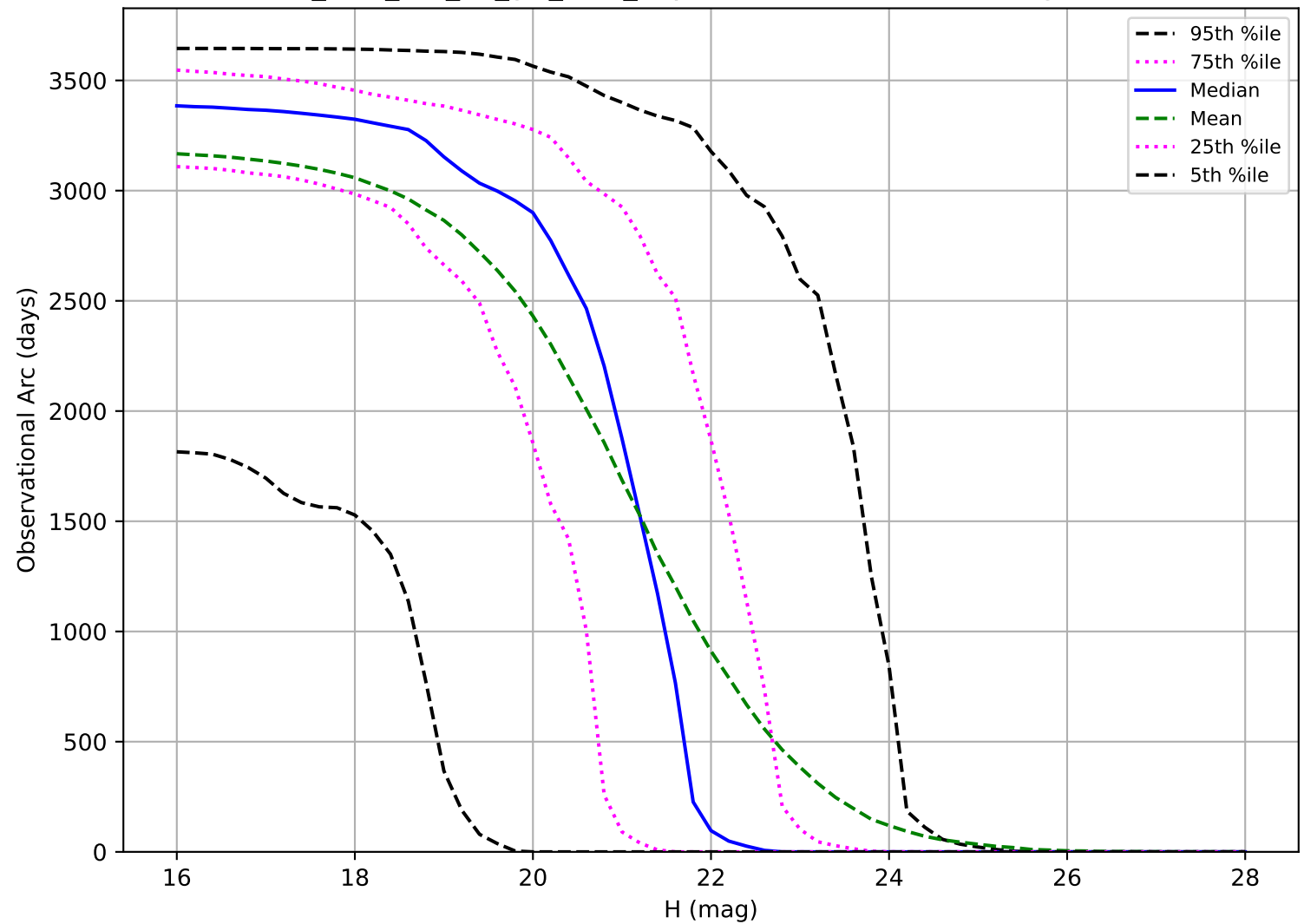
too_elab_r16_d2_giz_v3.4_10yrs: Observational Arc Length NEO
