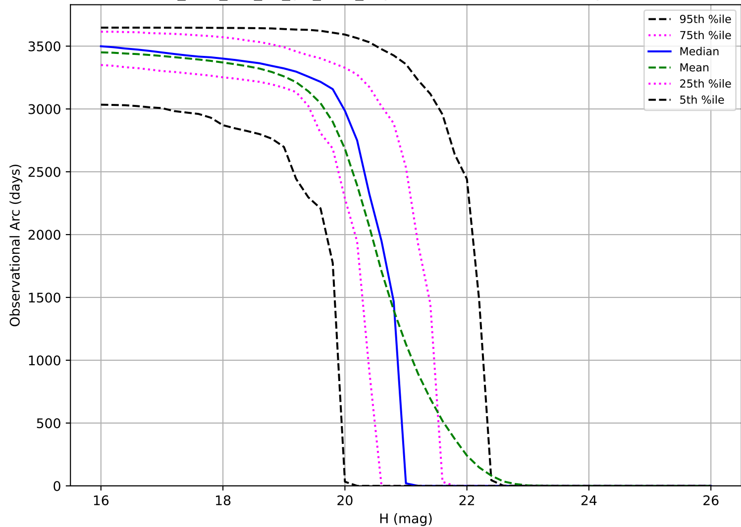
too_elab_r16_d2_giz_v3.4_10yrs: Observational Arc Length MBA
