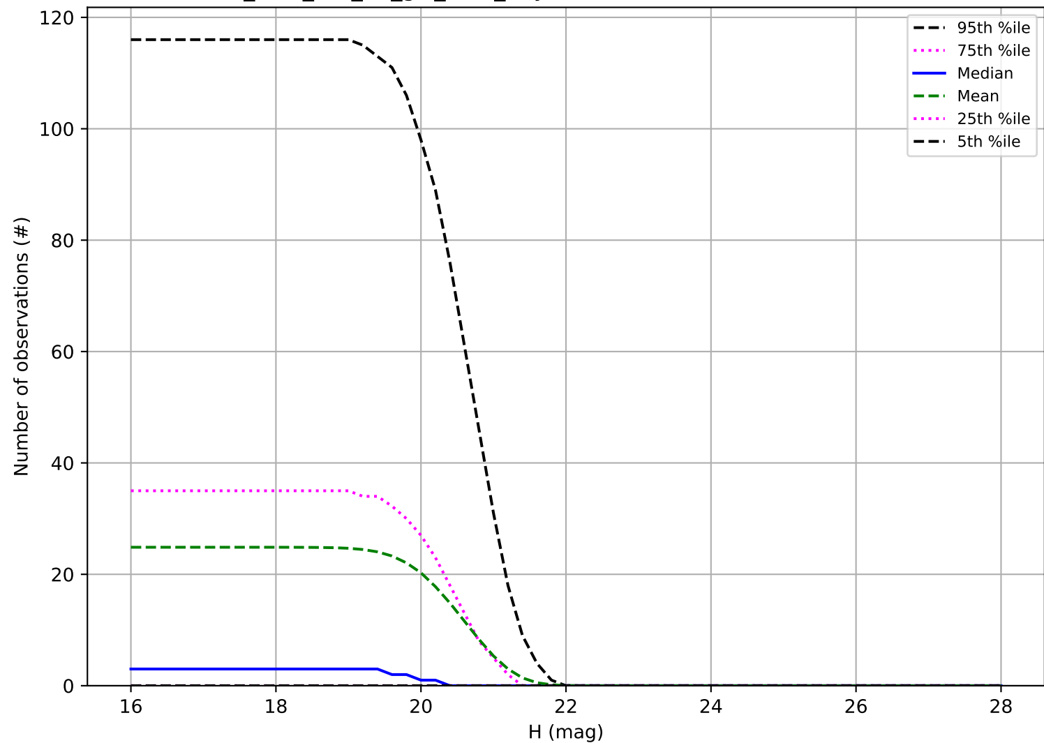
too_elab_r16_d2_giz_v3.4_10yrs: Number of observations Vatira
