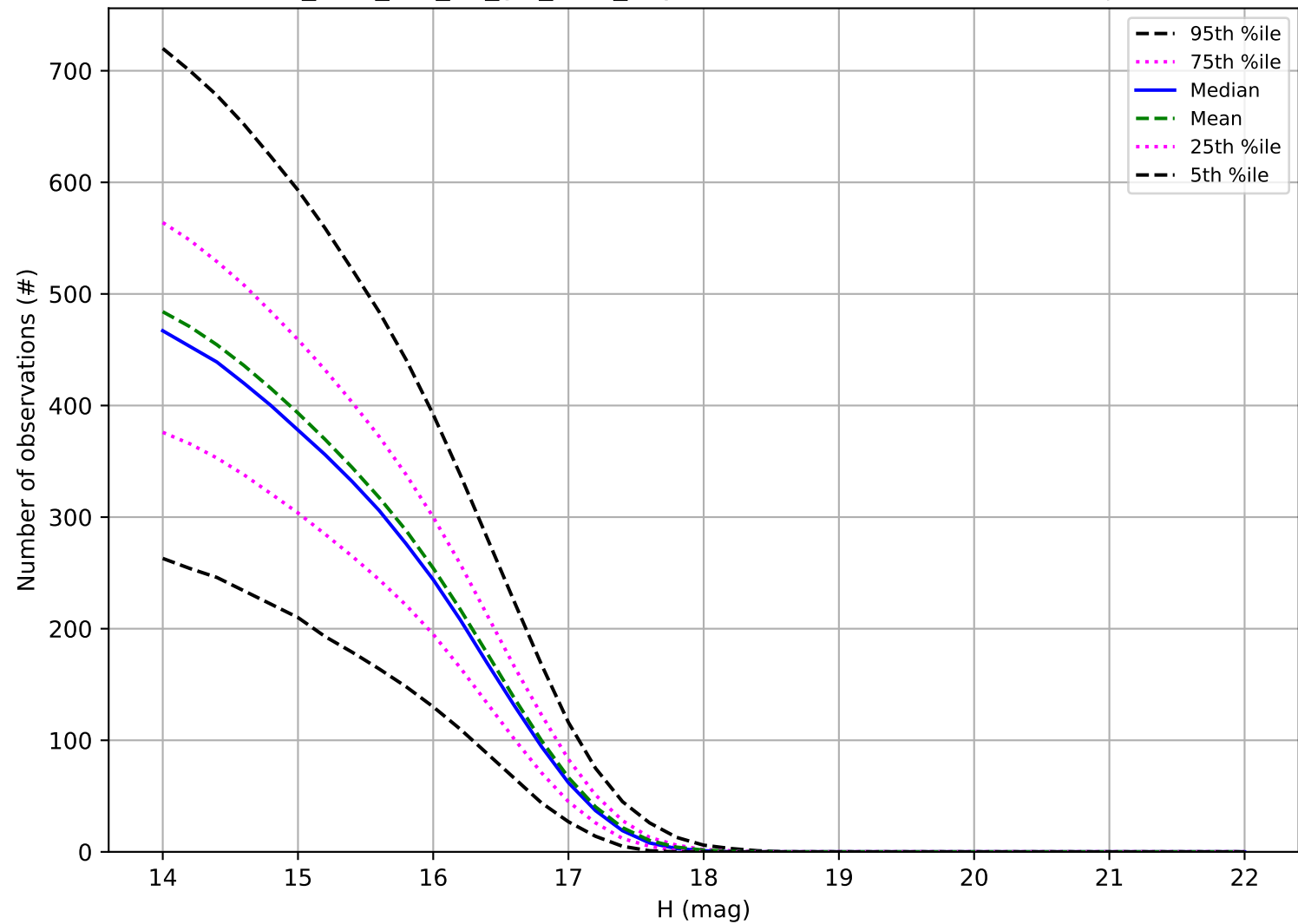
too_elab_r16_d2_giz_v3.4_10yrs: Number of observations Trojan
