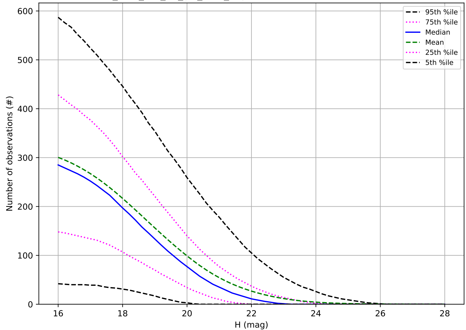
too_elab_r16_d2_giz_v3.4_10yrs: Number of observations PHA
