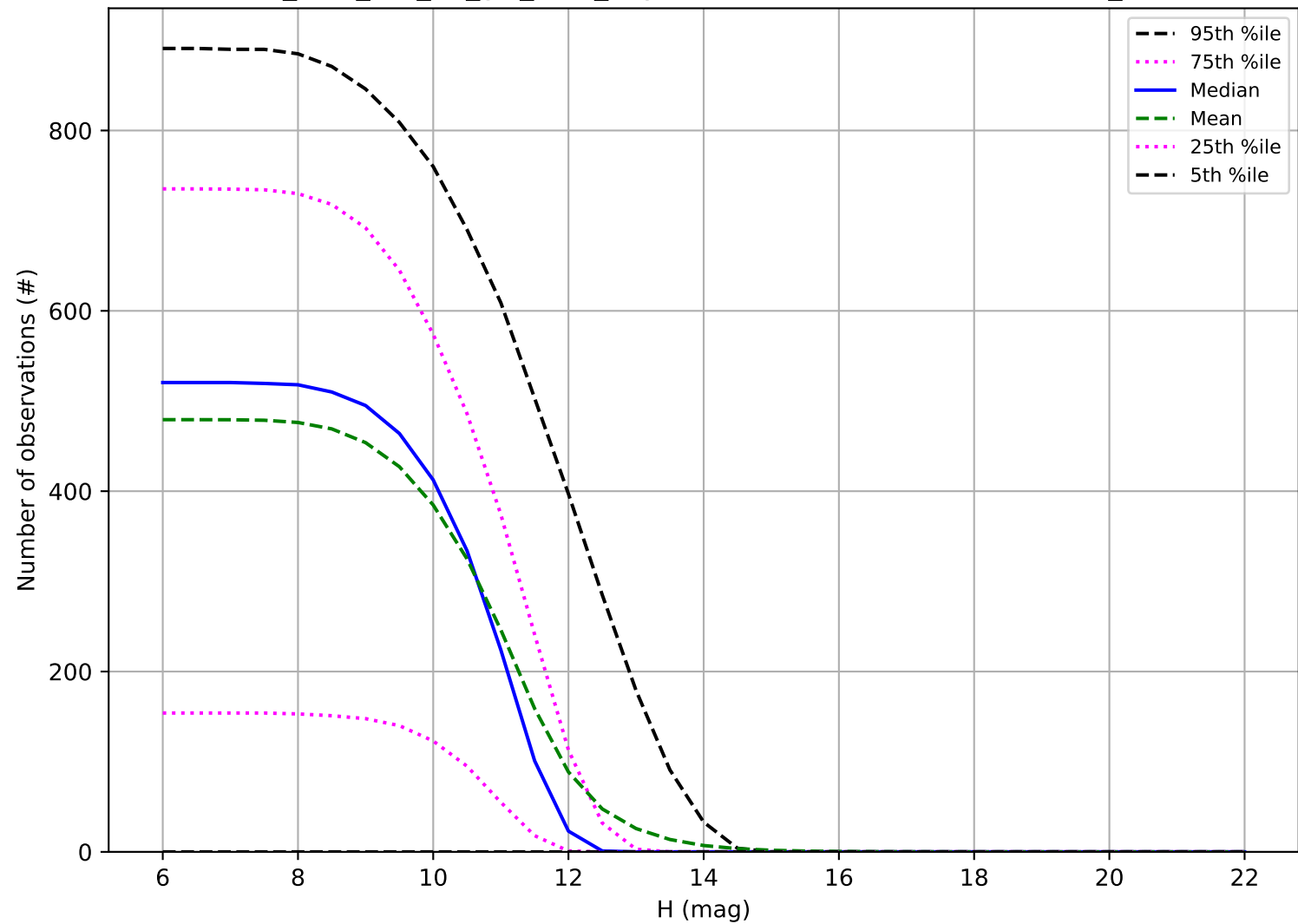
too_elab_r16_d2_giz_v3.4_10yrs: Number of observations OCC_r20
