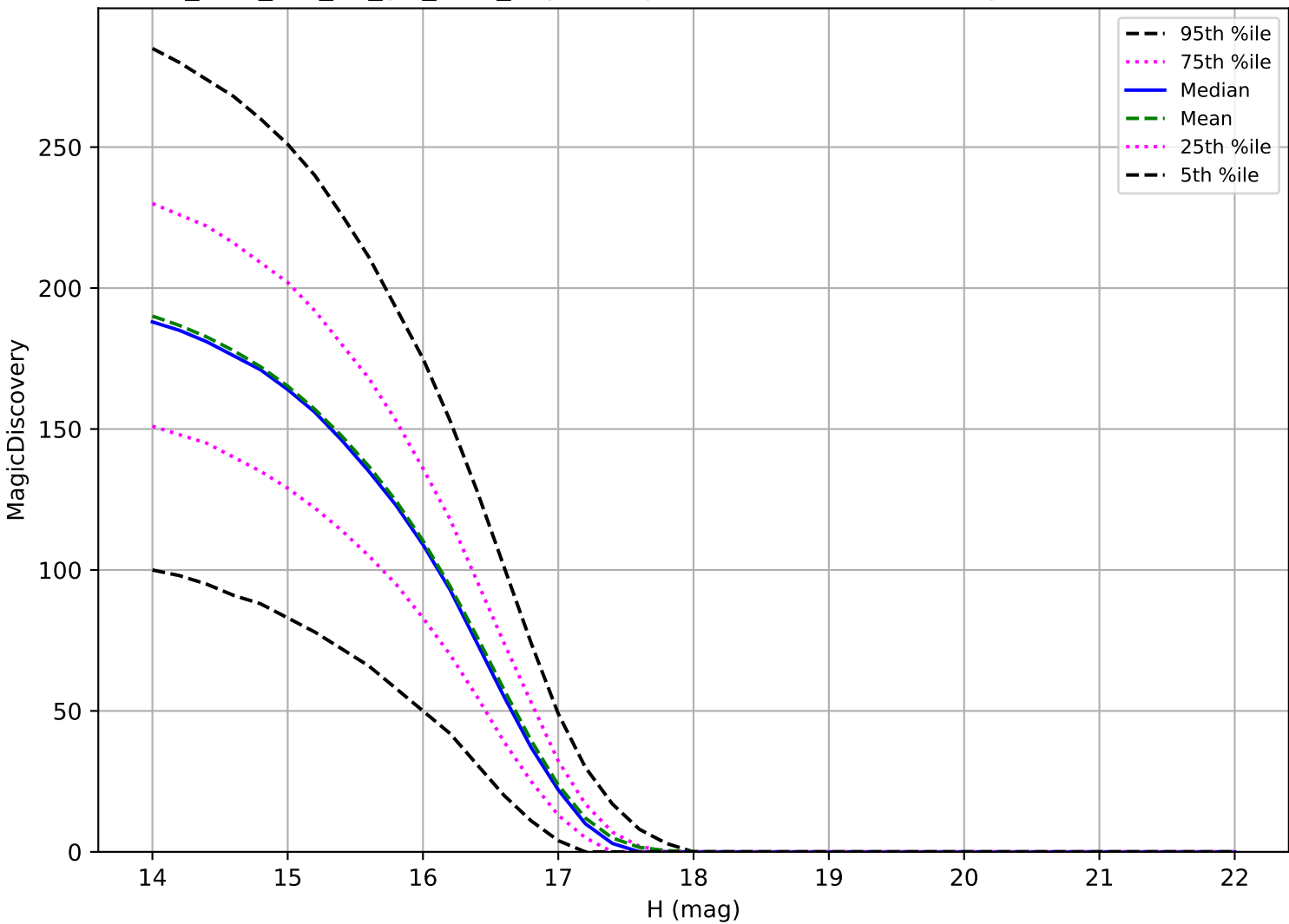
too_elab_r16_d2_giz_v3.4_10yrs: Trojan 6 detections in 60 nights detection loss
