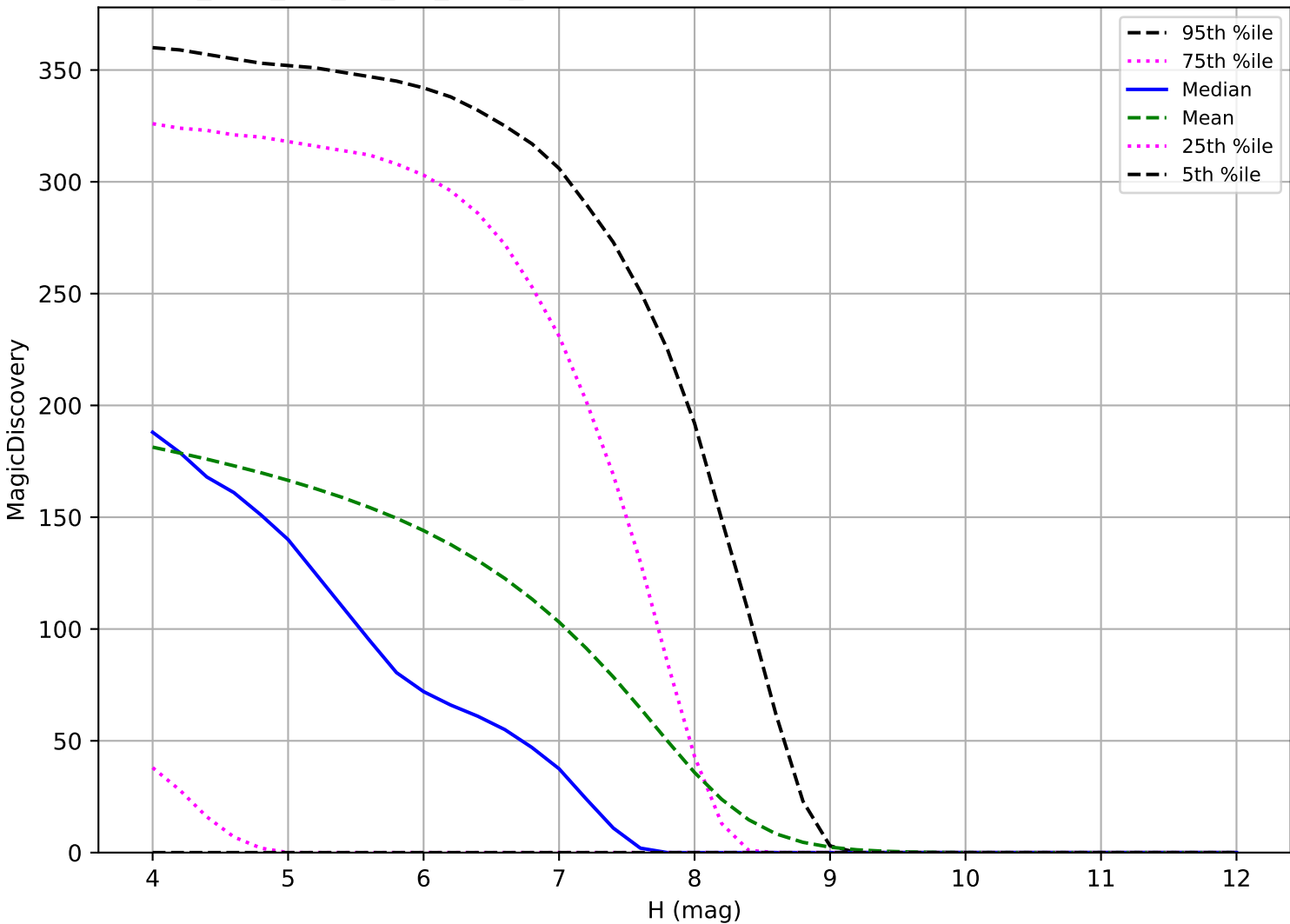
too_elab_r16_d2_giz_v3.4_10yrs: TNO 6 detections in 60 nights detection loss
