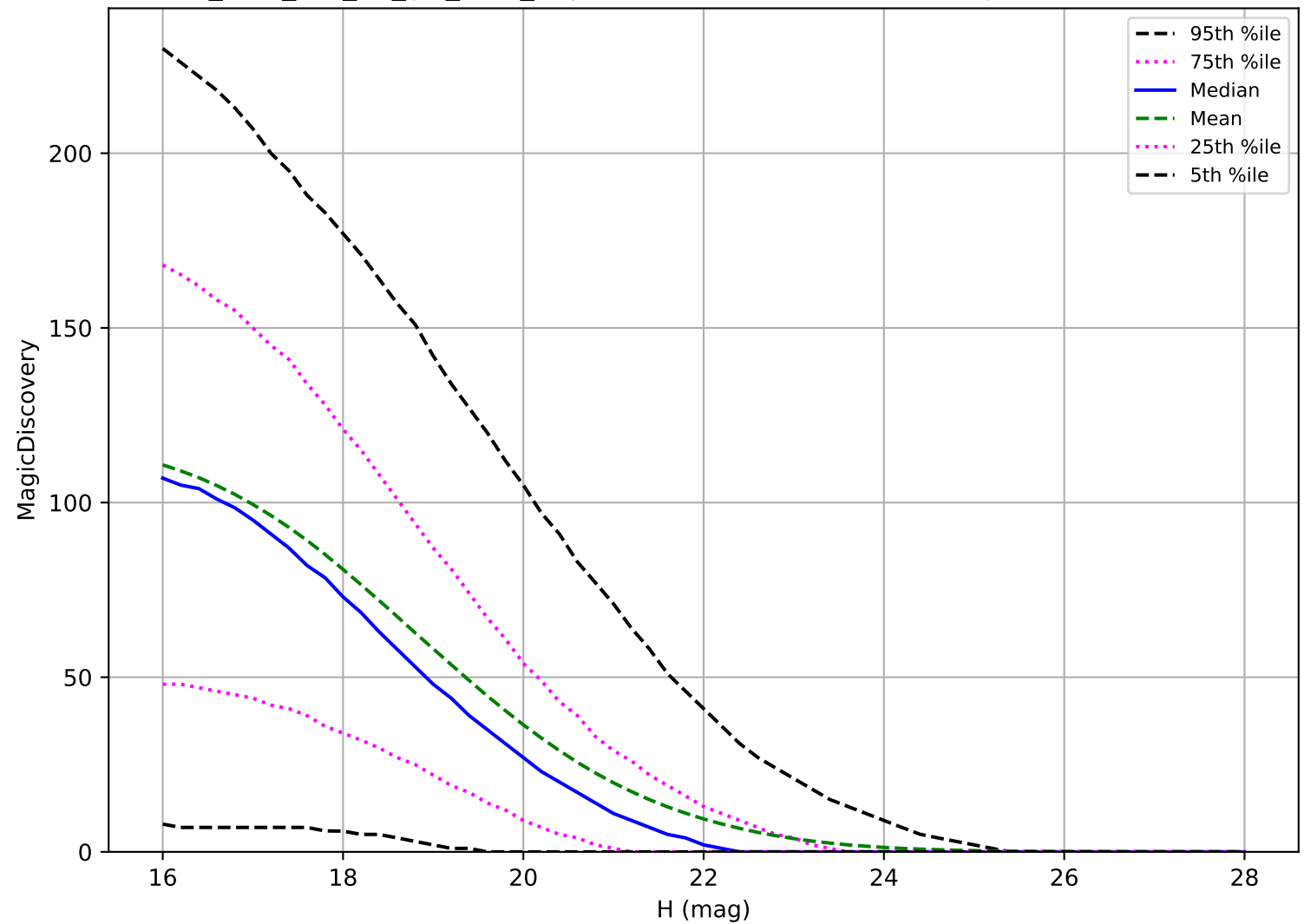
too_elab_r16_d2_giz_v3.4_10yrs: PHA 6 detections in 60 nights detection loss
