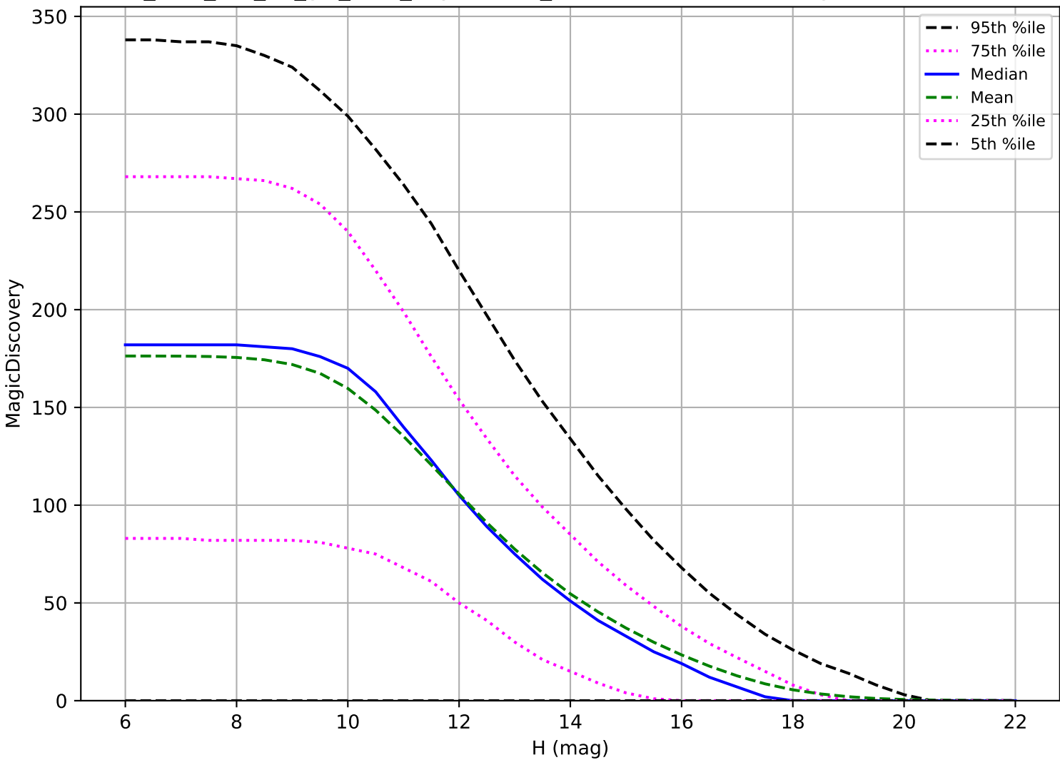
too_elab_r16_d2_giz_v3.4_10yrs: OCC_r5 6 detections in 60 nights detection loss
