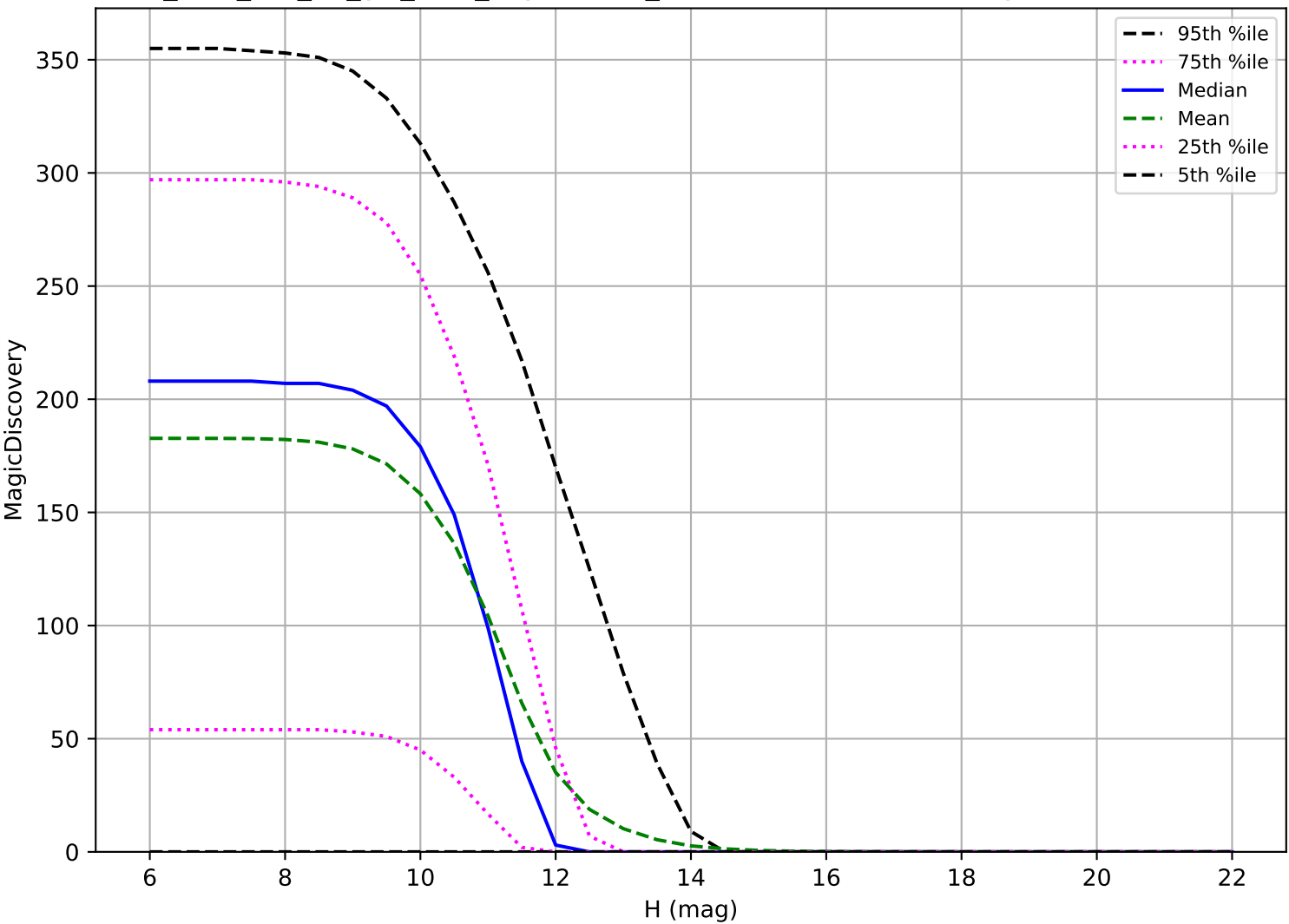
too_elab_r16_d2_giz_v3.4_10yrs: OCC_r20 6 detections in 60 nights detection loss
