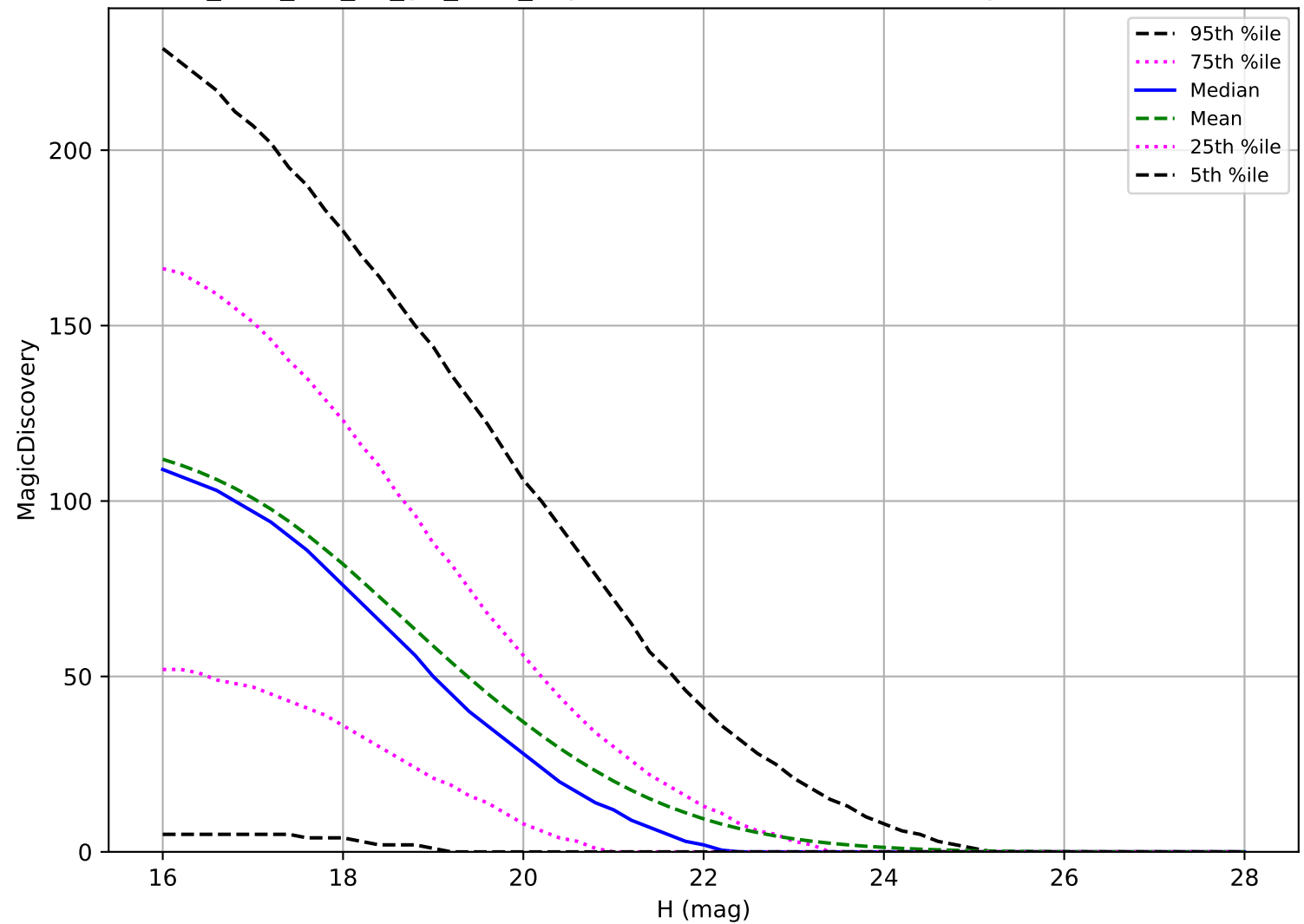
too_elab_r16_d2_giz_v3.4_10yrs: NEO 6 detections in 60 nights detection loss
