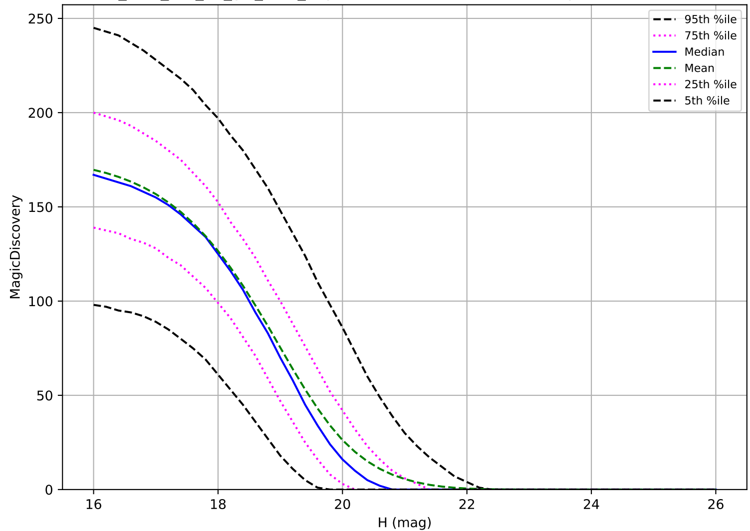
too_elab_r16_d2_giz_v3.4_10yrs: MBA 6 detections in 60 nights detection loss
