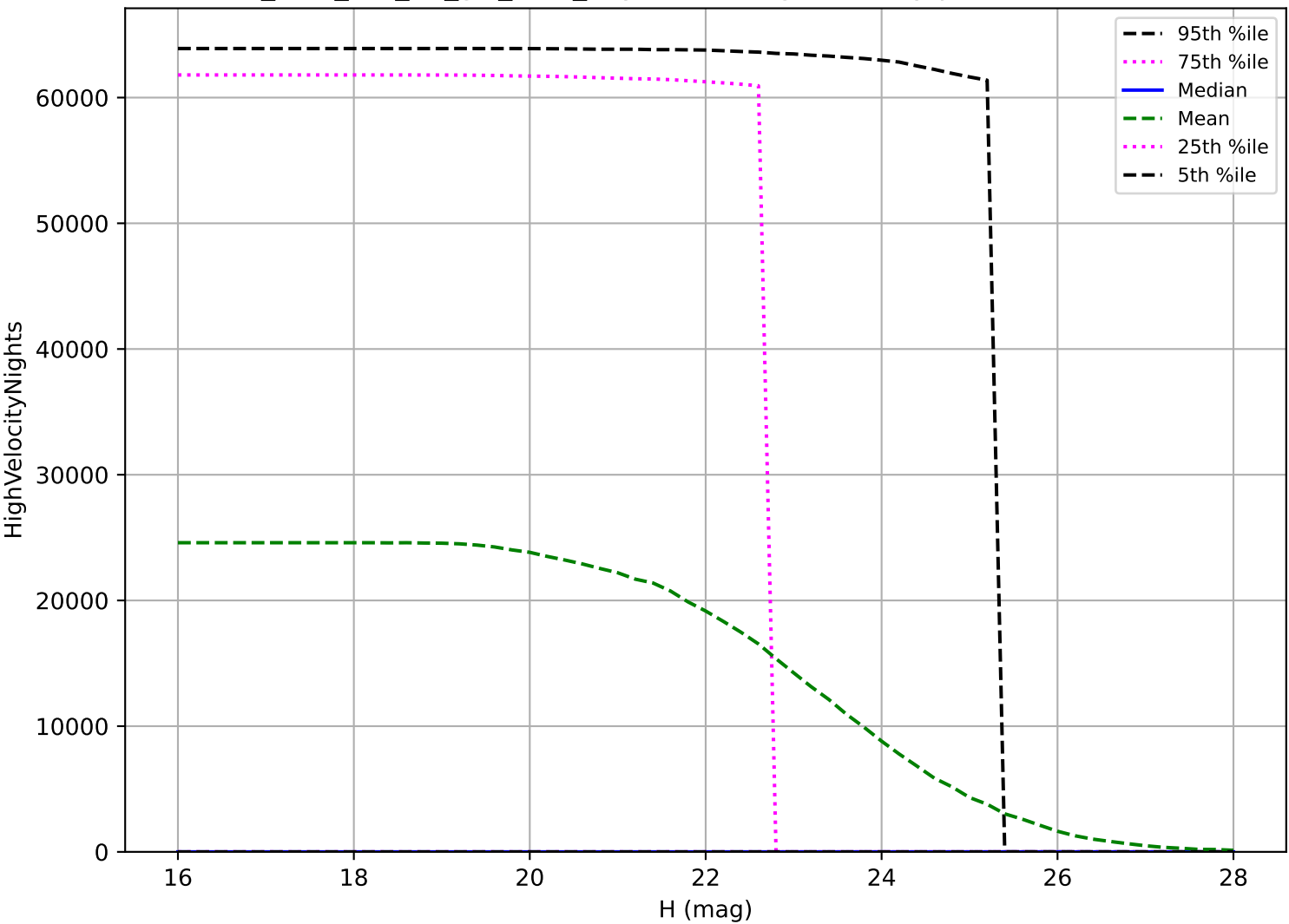
too_elab_r16_d2_giz_v3.4_10yrs: PHA High velocity pair detection loss
