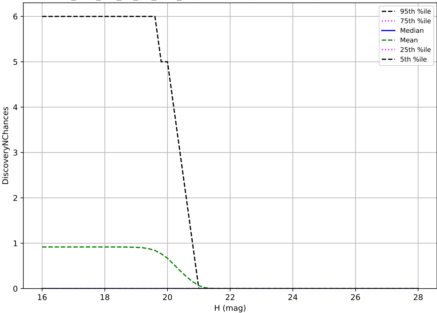
too_elab_r16_d2_giz_v3.4_10yrs: Vatira 3 pairs in 15 nights detection loss
