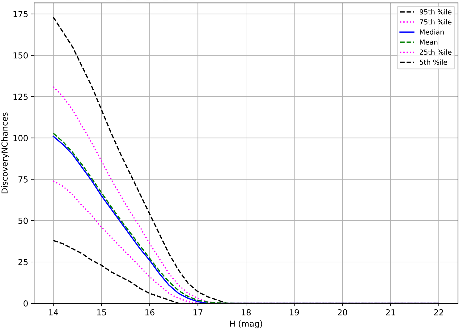
too_elab_r16_d2_giz_v3.4_10yrs: Trojan 3 pairs in 15 nights detection loss
