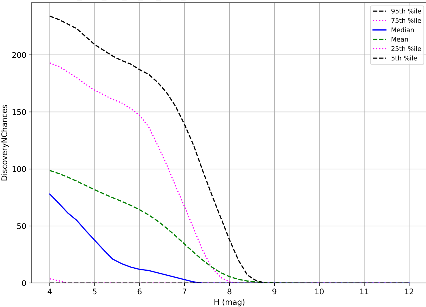
too_elab_r16_d2_giz_v3.4_10yrs: TNO 3 pairs in 15 nights detection loss
