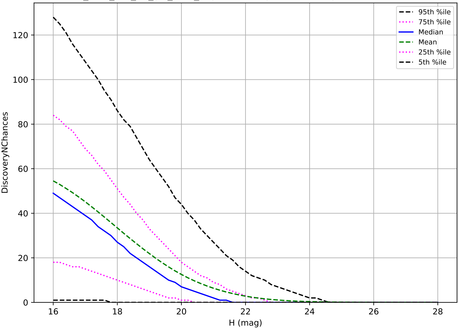
too_elab_r16_d2_giz_v3.4_10yrs: PHA 3 pairs in 15 nights detection loss
