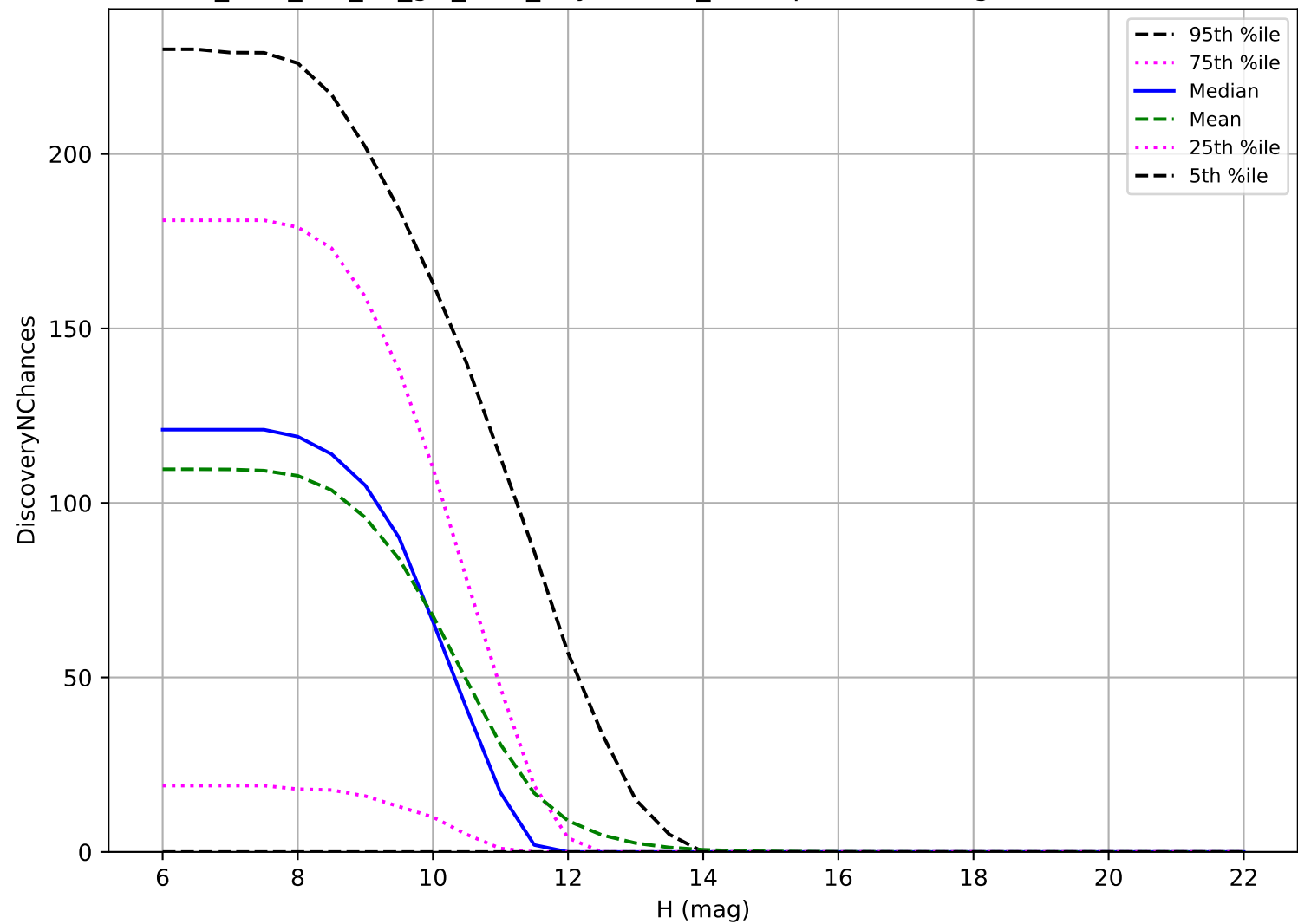
too_elab_r16_d2_giz_v3.4_10yrs: OCC_r20 3 pairs in 15 nights detection loss
