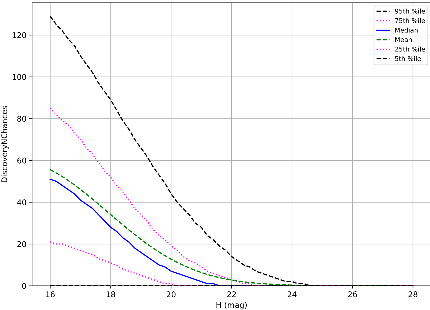
too_elab_r16_d2_giz_v3.4_10yrs: NEO 3 pairs in 15 nights detection loss
