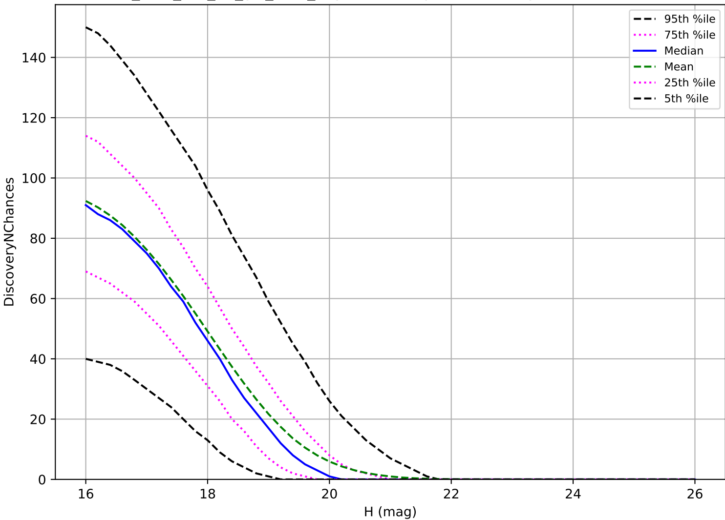
too_elab_r16_d2_giz_v3.4_10yrs: MBA 3 pairs in 15 nights detection loss
