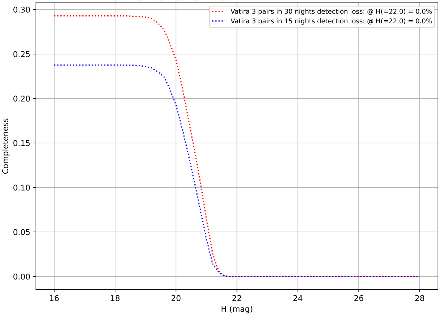
too_elab_r16_d2_giz_v3.4_10yrs: DifferentialCompleteness
