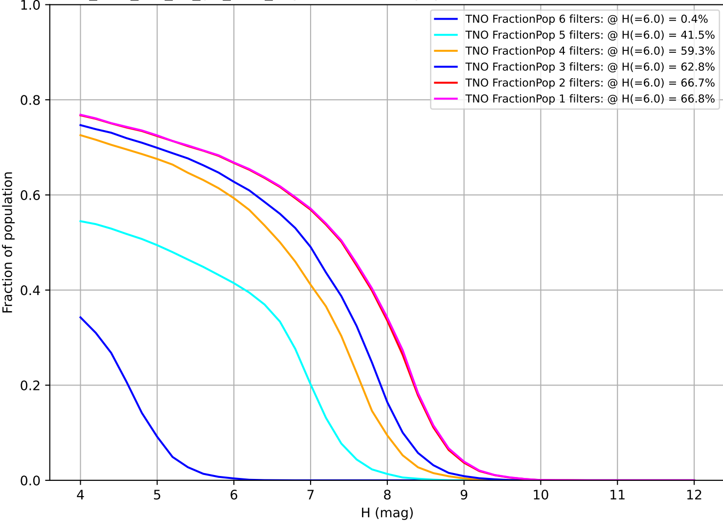
too_elab_r16_d2_giz_v3.4_10yrs: Fraction of population with colors in X filters TNO
