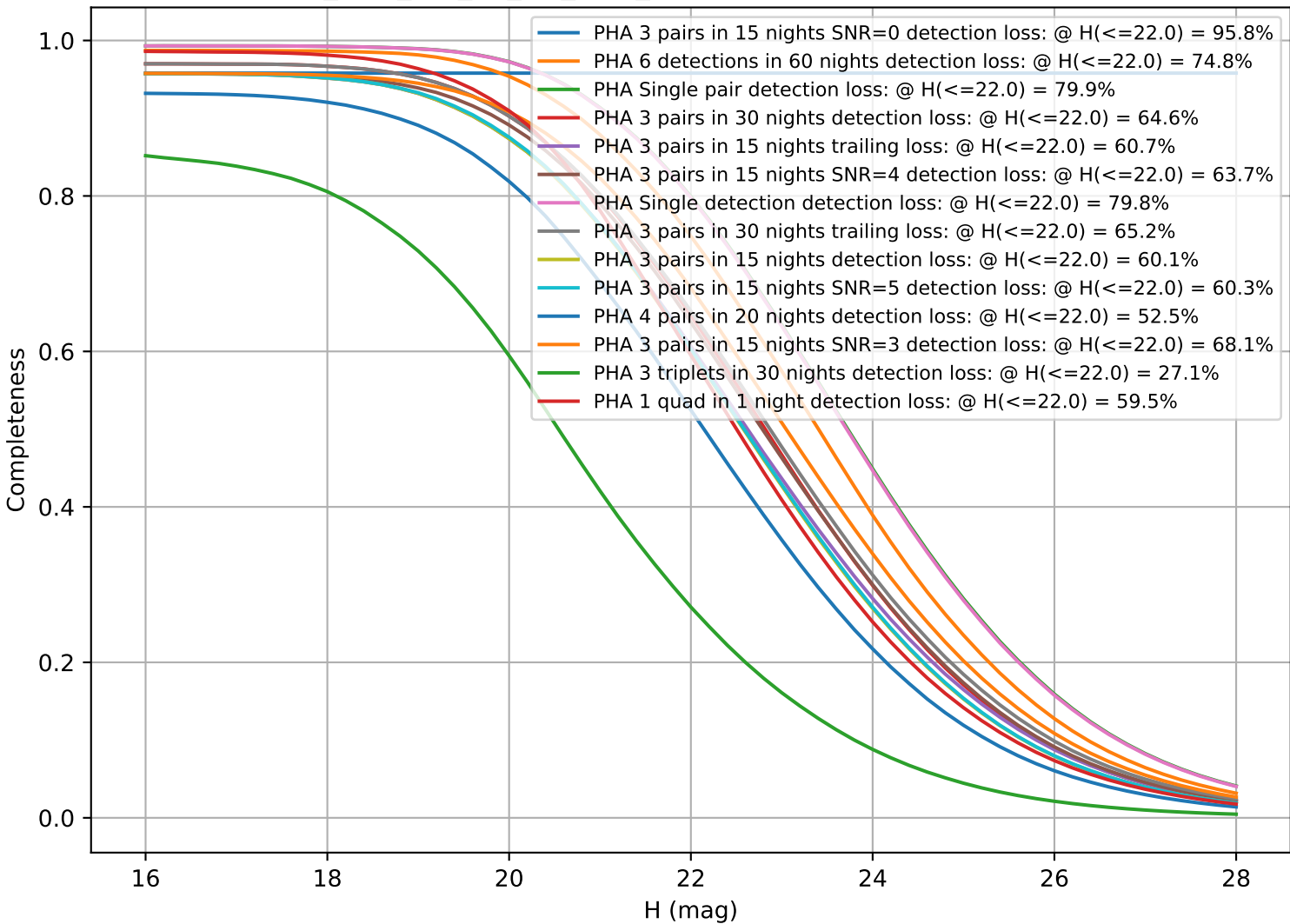
too_elab_r16_d2_giz_v3.4_10yrs: CumulativeCompleteness
