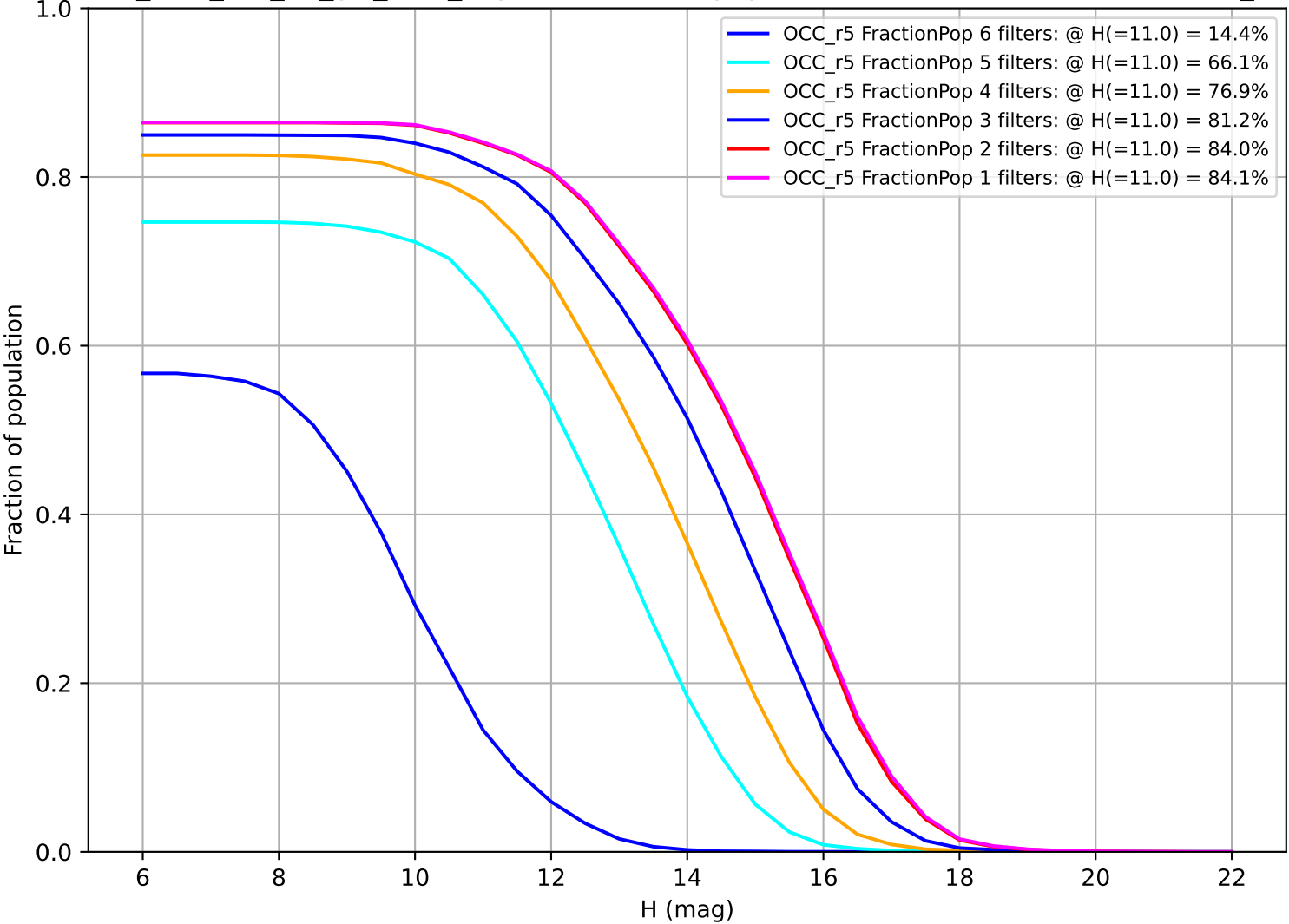
too_elab_r16_d2_giz_v3.4_10yrs: Fraction of population with colors in X filters OCC_r5
