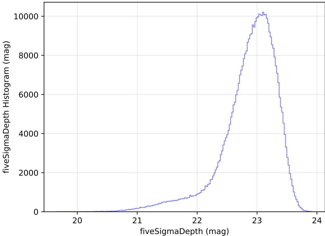
too_elab_r16_d2_giz_v3.4_10yrs z: fiveSigmaDepth Histogram
