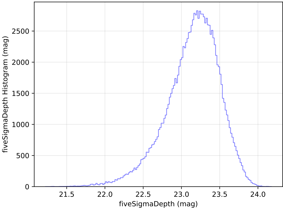
too_elab_r16_d2_giz_v3.4_10yrs u: fiveSigmaDepth Histogram
