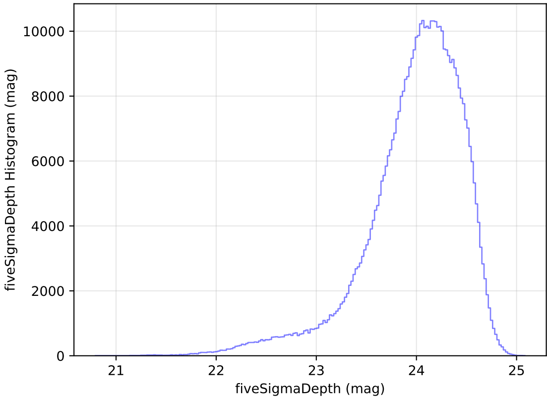
too_elab_r16_d2_giz_v3.4_10yrs r: fiveSigmaDepth Histogram
