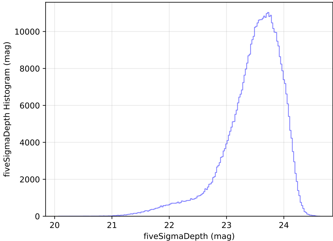
too_elab_r16_d2_giz_v3.4_10yrs i: fiveSigmaDepth Histogram
