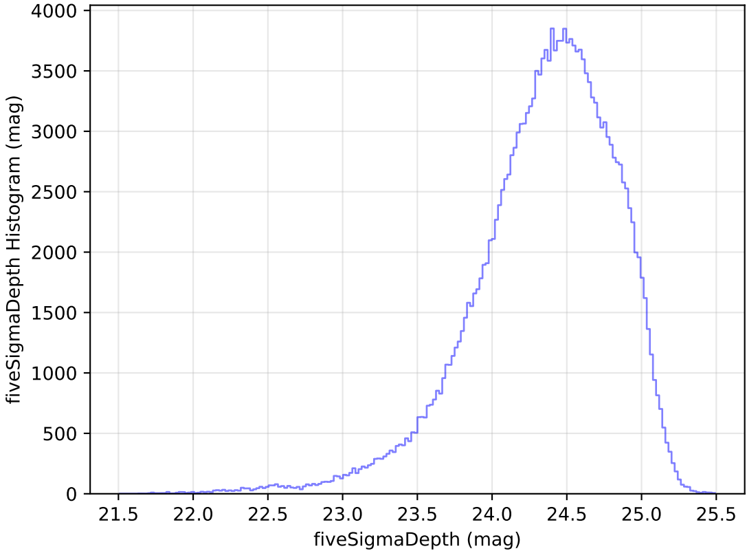
too_elab_r16_d2_giz_v3.4_10yrs g: fiveSigmaDepth Histogram
