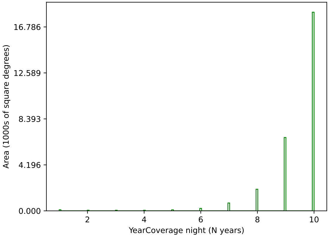
too_elab_r16_d2_giz_v3.4_10yrs g band: YearCoverage night
