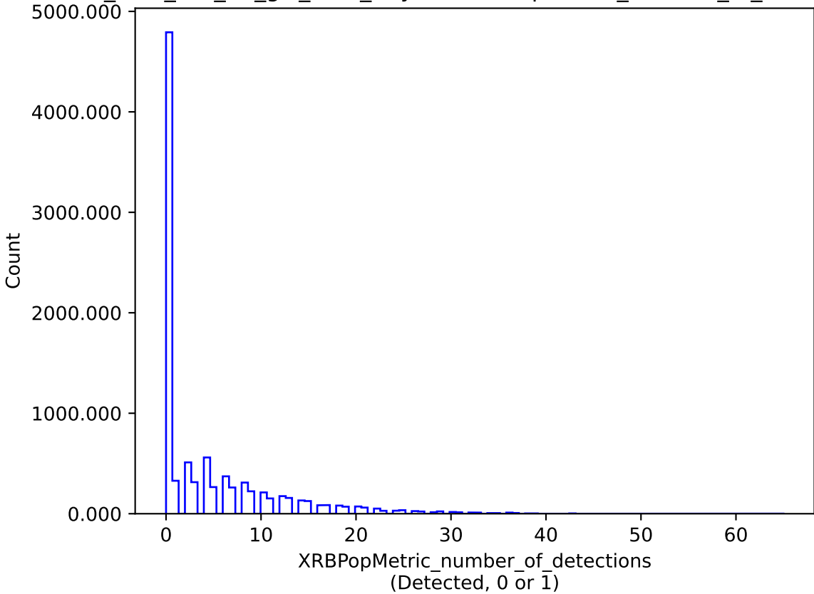
too_elab_r16_d2_giz_v3.4_10yrs : XRBPopMetric_number_of_detections
