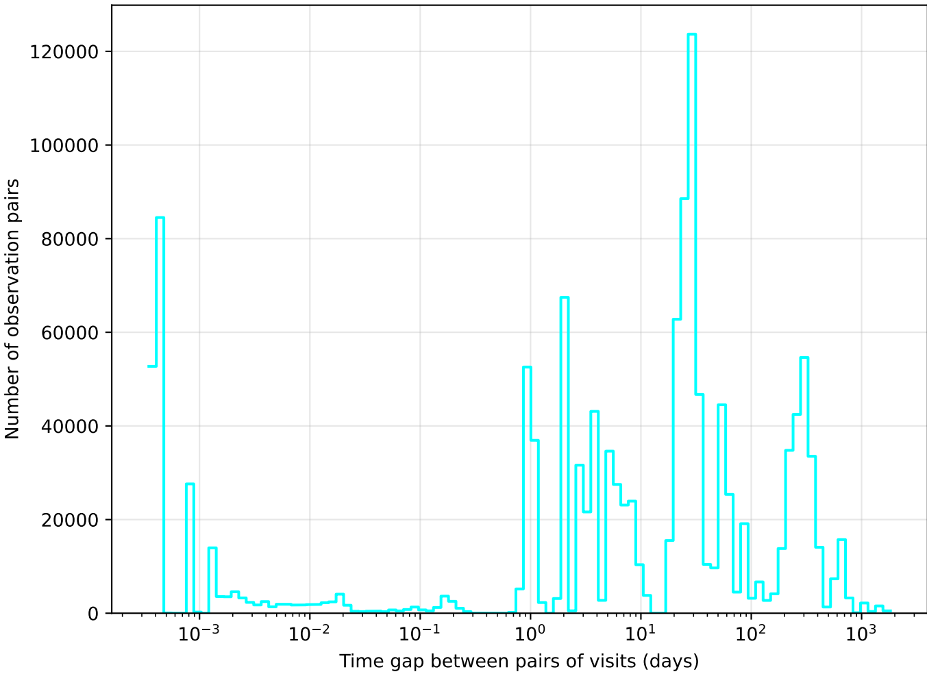
too_elab_r16_d2_giz_v3.4_10yrs u band: Tgaps observationStartMJD
