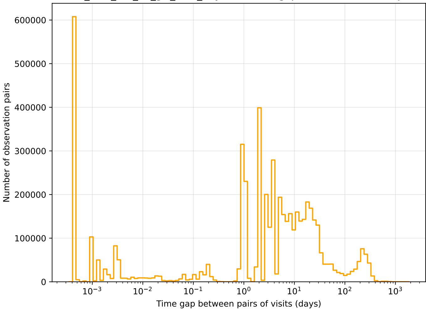
too_elab_r16_d2_giz_v3.4_10yrs r band: Tgaps observationStartMJD
