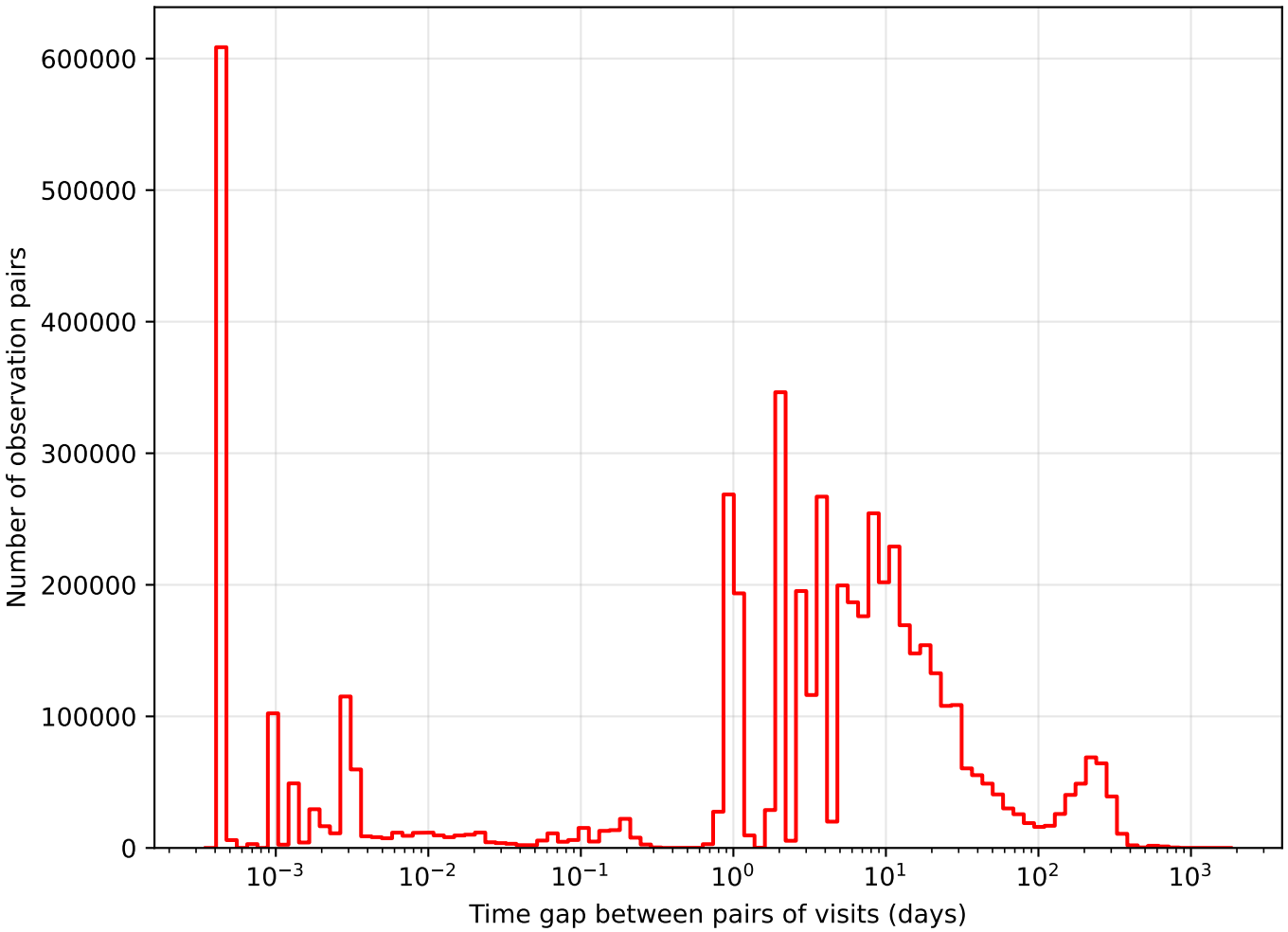
too_elab_r16_d2_giz_v3.4_10yrs i band: Tgaps observationStartMJD
