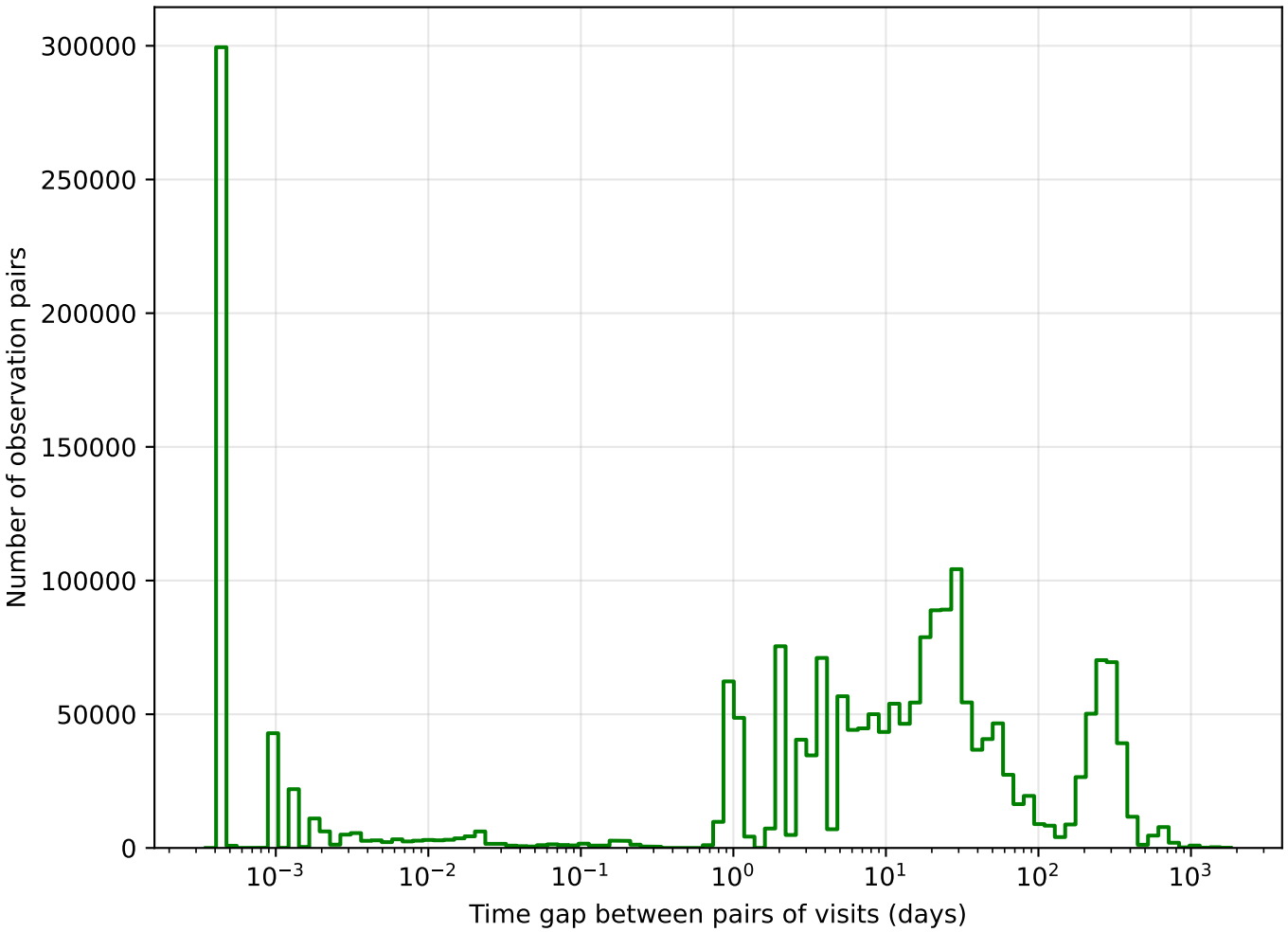
too_elab_r16_d2_giz_v3.4_10yrs g band: Tgaps observationStartMJD
