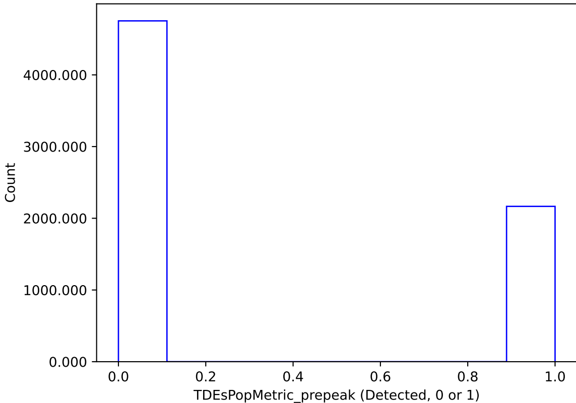
too_elab_r16_d2_giz_v3.4_10yrs : TDEsPopMetric_prepeak
