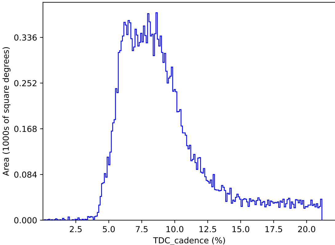
too_elab_r16_d2_giz_v3.4_10yrs : TDC_cadence
