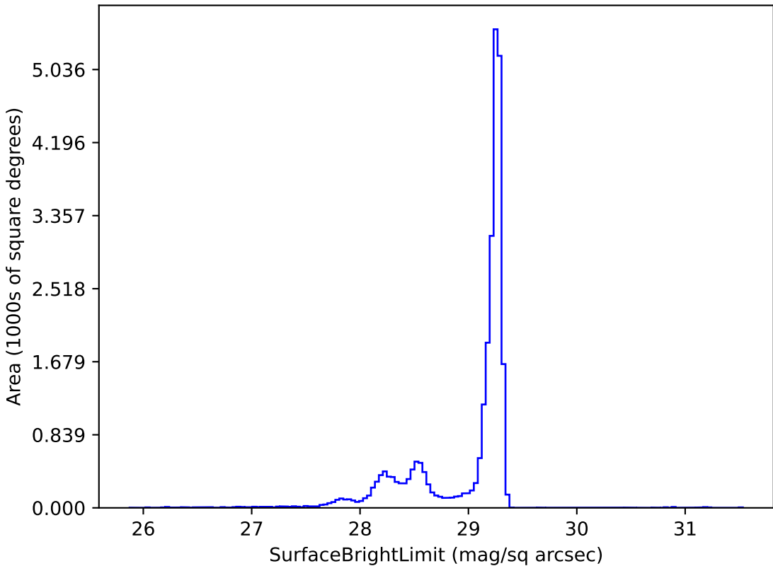
too_elab_r16_d2_giz_v3.4_10yrs z: SurfaceBrightLimit
