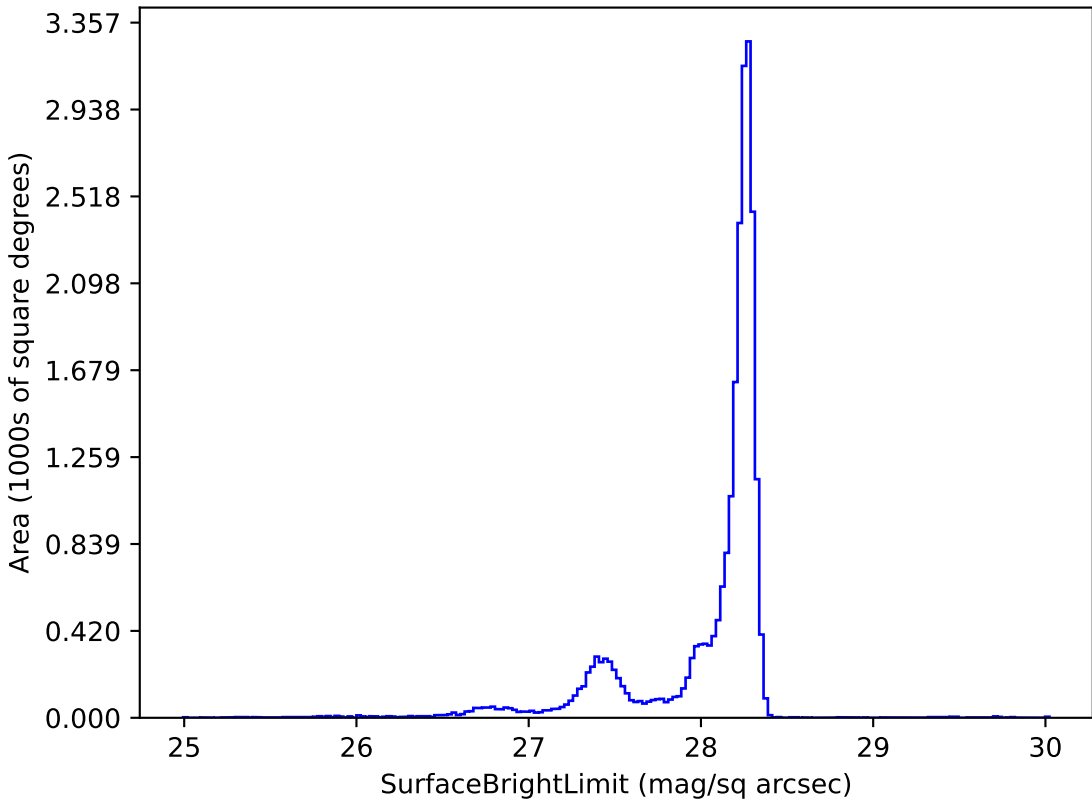
too_elab_r16_d2_giz_v3.4_10yrs y: SurfaceBrightLimit
