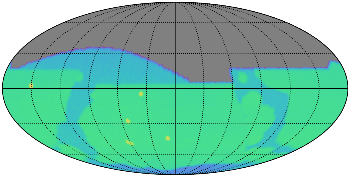
too_elab_r16_d2_giz_v3.4_10yrs r: SurfaceBrightLimit
