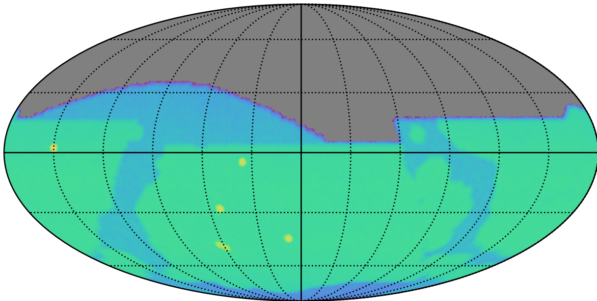
too_elab_r16_d2_giz_v3.4_10yrs i: SurfaceBrightLimit
