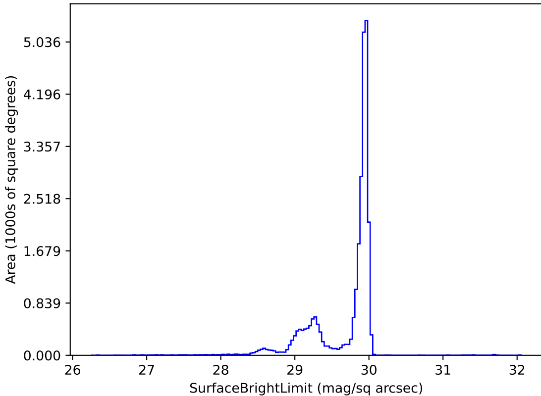
too_elab_r16_d2_giz_v3.4_10yrs i: SurfaceBrightLimit
